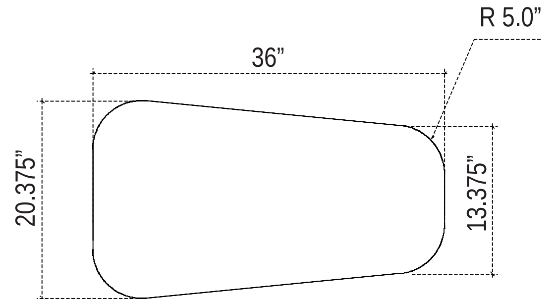
Trapezoid Header
